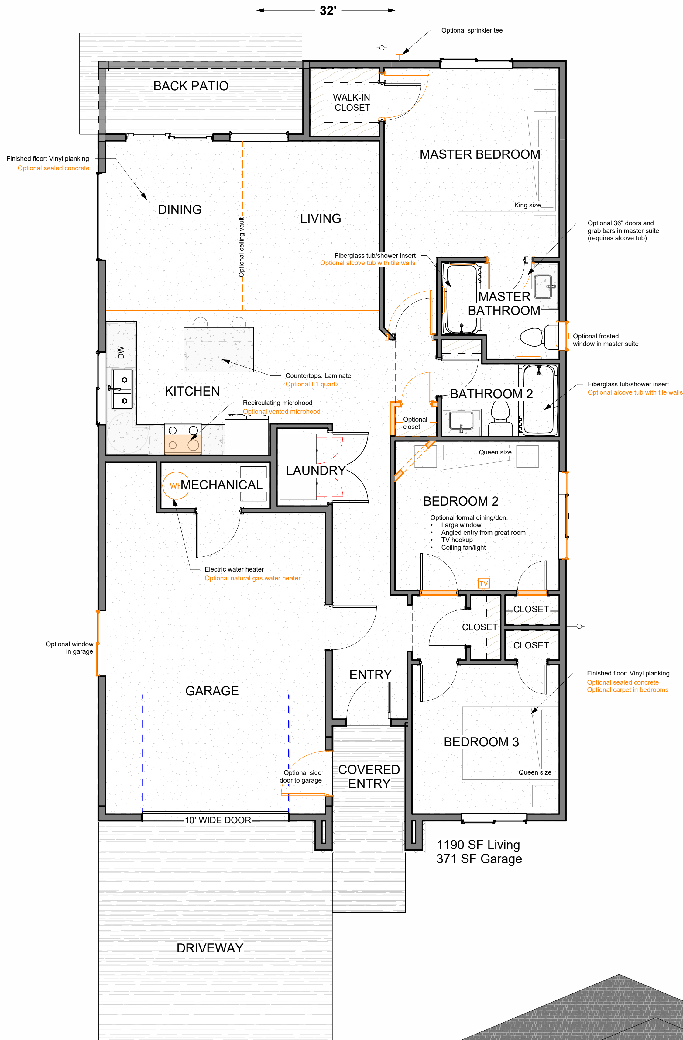
① Layout 1/4" = 1'-0"
